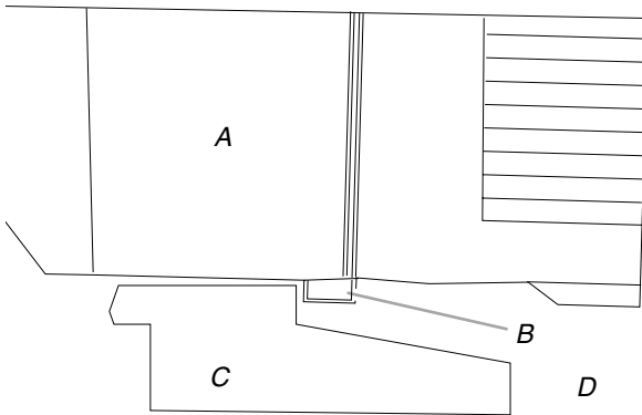
A. Air conditioner B. Bottom channel C. Windowsill D. Outside
